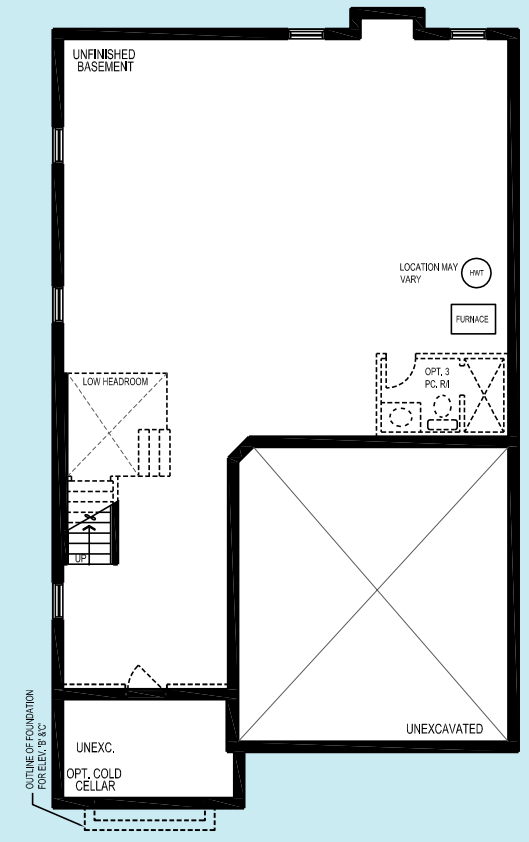
LOWER LEVEL STYLE A, B & C
